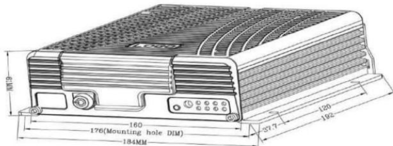
General Dimensions
